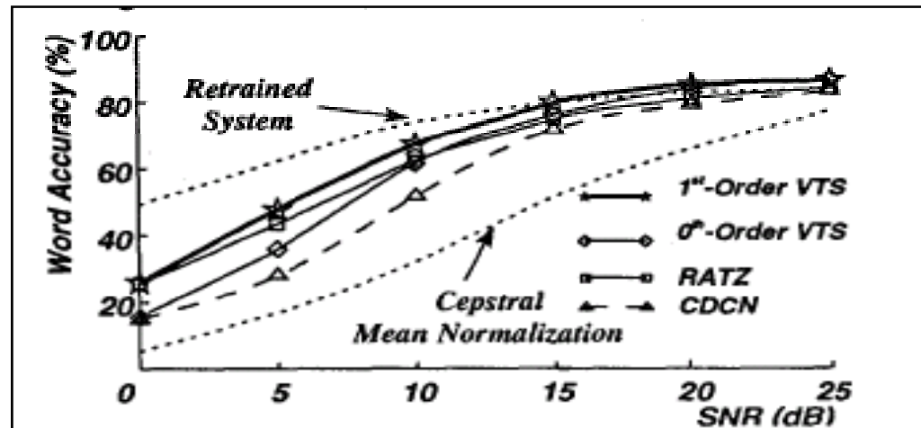
Figure 3. Comparison of recognition accuracy obtained for the CENSUS database using the zeroth-order and first-order VTS, CDCN, and RATZ algorithms as a function of SNR. The dotted curves indicate baseline performance using cepstral mean normalization only, as well as results obtained by completely retraining the system in the new environment.
